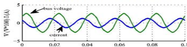
Fig. 8. DPFC operation in steady state: bus voltage and current at the \Delta side of the transformer
