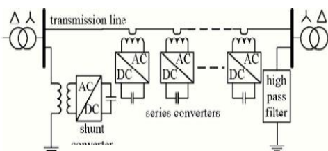
Fig. 2. DPFC configuration
