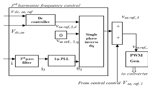
Fig.3 Block diagram of series converter control
