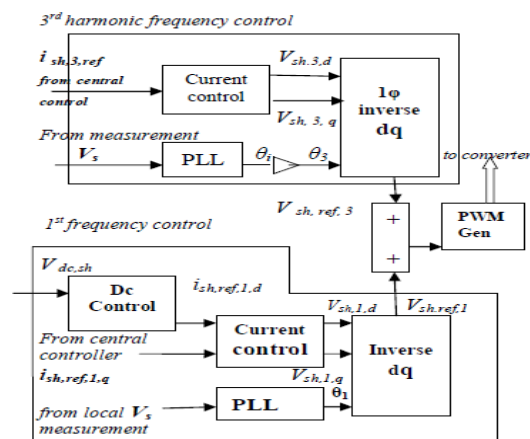
Fig.4 Block diagram of shunt converter control
