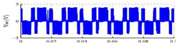
Fig. 7. DPFC operation in steady state: series converter voltage
