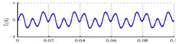
Fig. 6. DPFC operation in steady state line current
