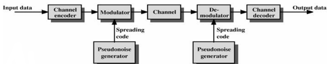
Fig. 1: Spread Spectrum
