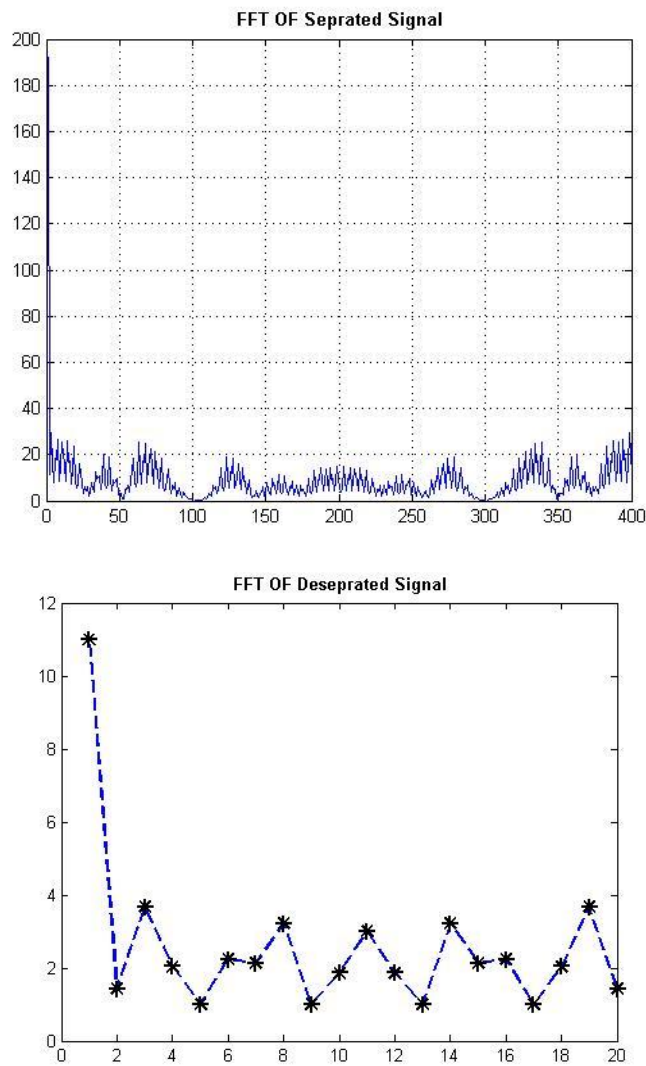
Fig.11. Waveforms for FFT for Separated and Despread Signals
