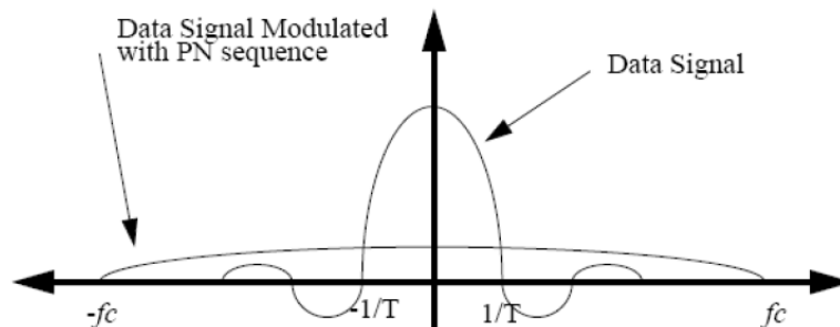
Fig. 3:Data Signal and PN signal in Frequency Domain
