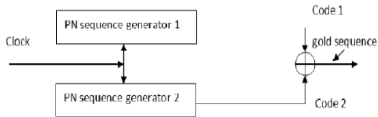
Fig.5.Gold Code Generator
