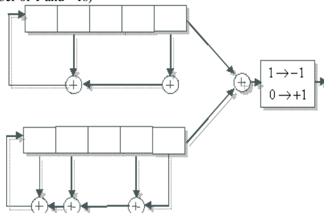
Fig.4: Gold sequence generator using one preferred pair of m -sequences
