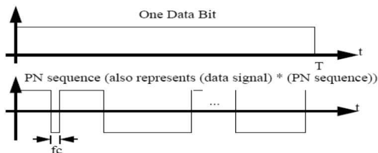
Fig. 2: Data Signal and PN signal in Time Domain.
