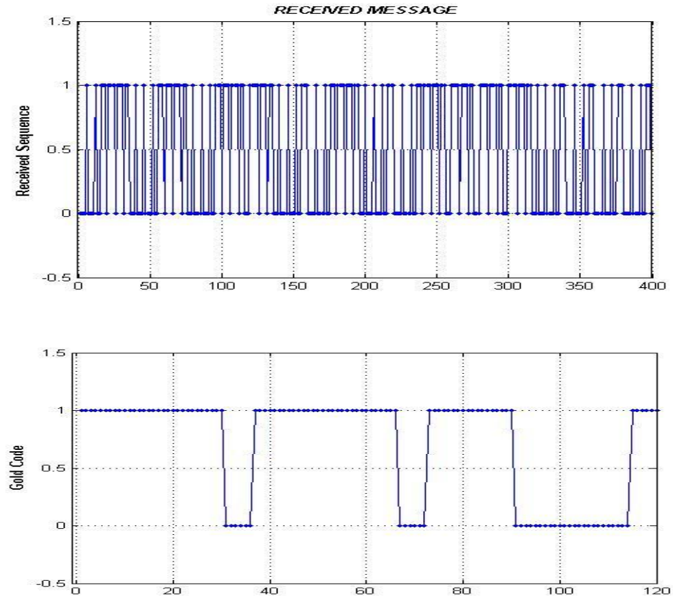
Fig.9. Waveforms for the Modulation Process
