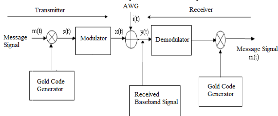
Figure 8 depicts transmitter, channel and receiver of DSSS system.
